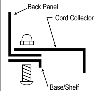
Figure C: Add a shelf
